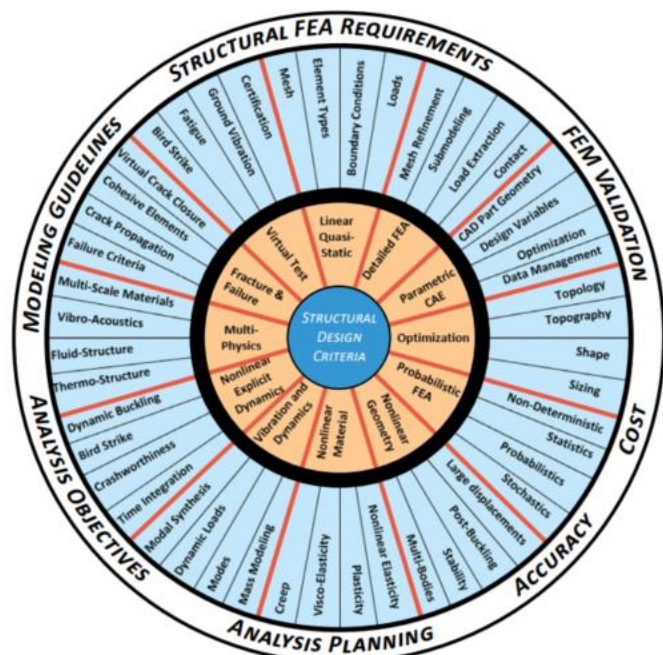
Figure 1 Boeing Structural Design Criteria Chart
