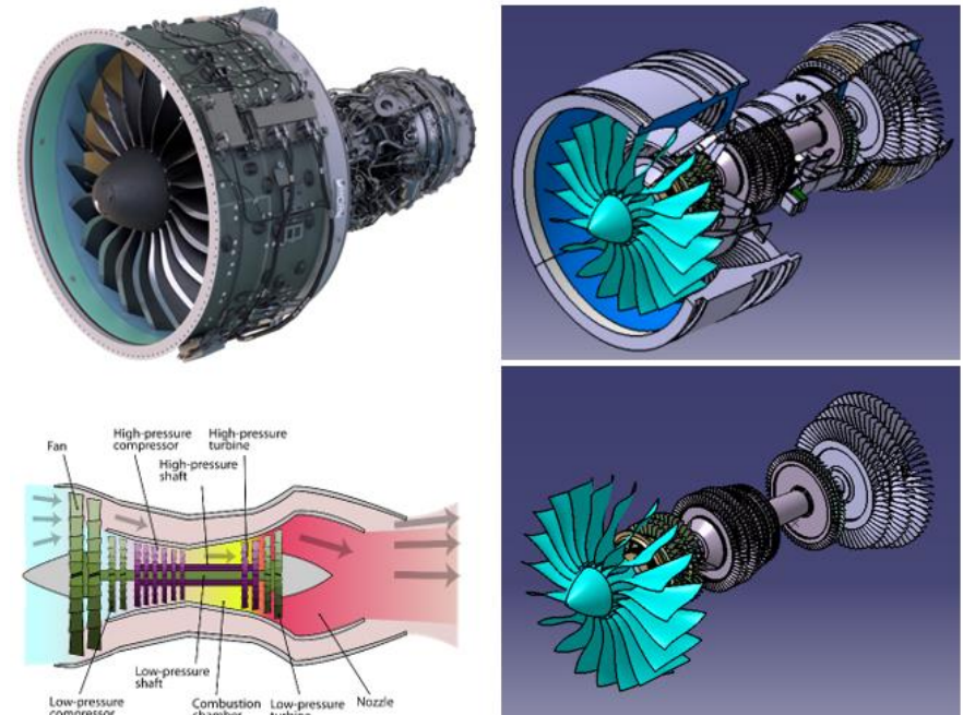
Figure 2 Example Turbofan Engine: Pratt & Whitney PW1000G
