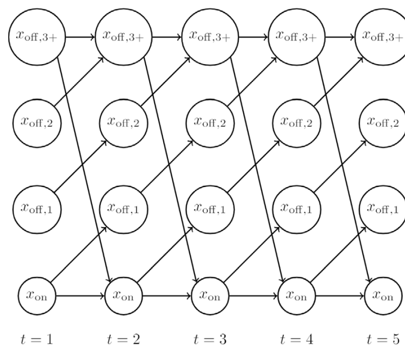
State transition graph corresponding to the ED problem for gas turbines
