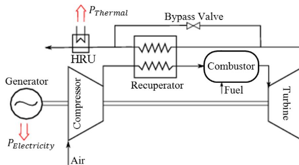
Engine schematic cycle
