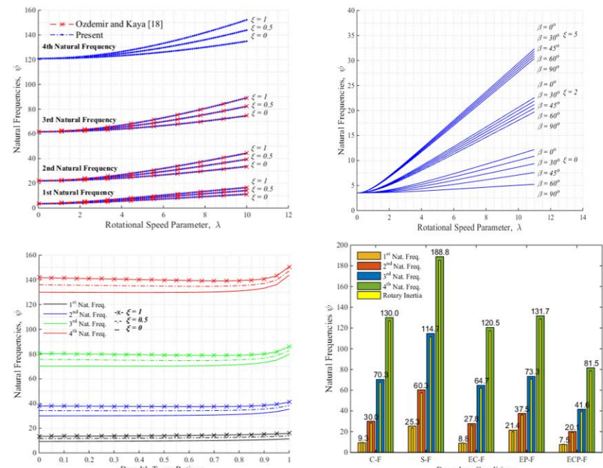
Figure 4 Nondimensional Natural Frequencies of the Blades
