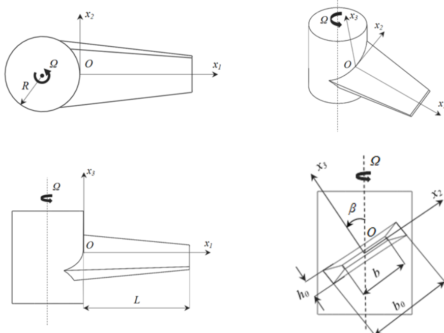
Figure 3 Simplified Turbofan Blades as Beam Elements
